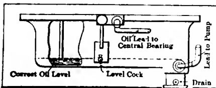
Fig. 6—The crankcase of the S. G. V. car, illustrating the oil well in the rear end to provide section for the pump
